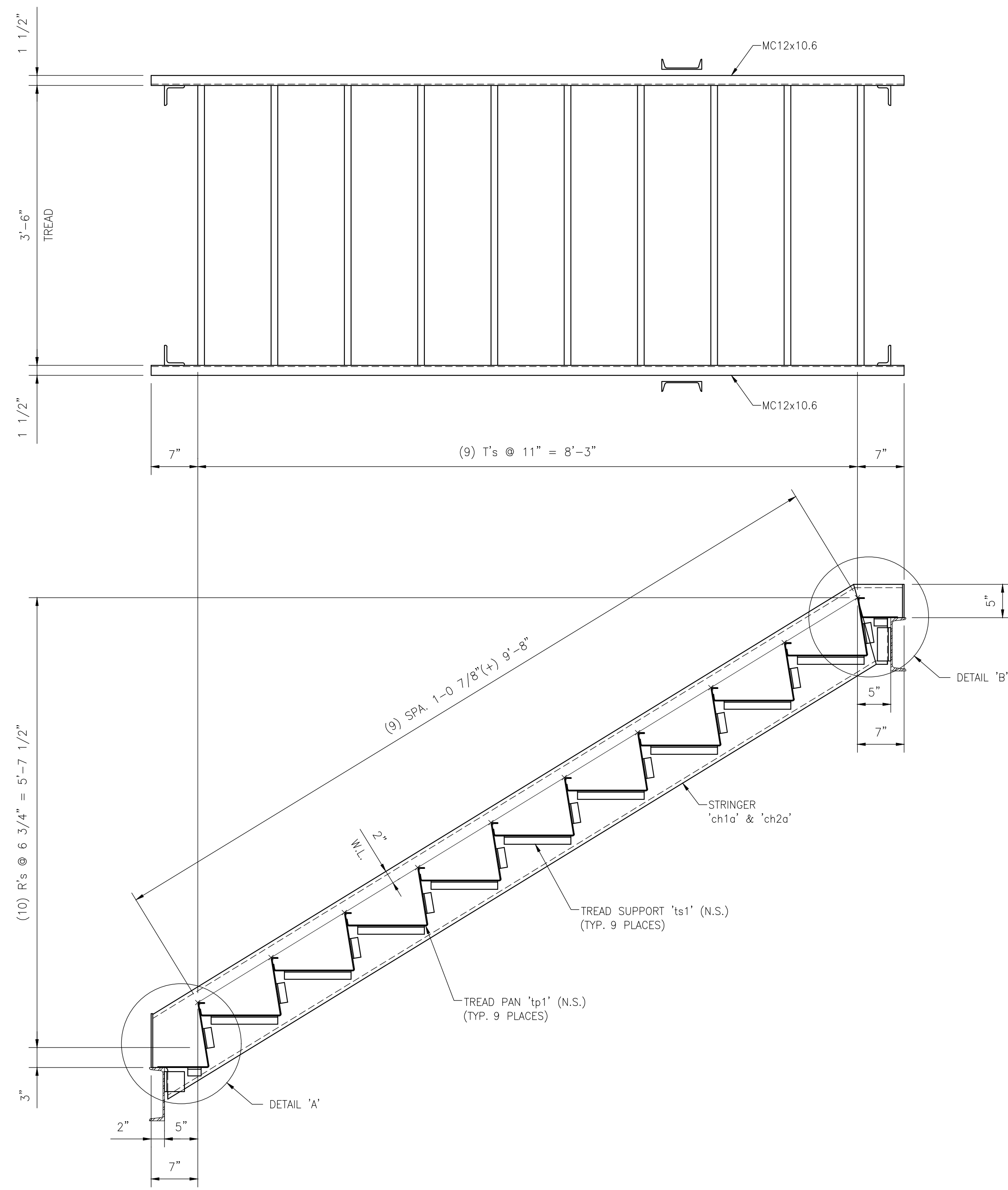
'7SA' - STAIR ASSEMBLY - 10 REQUIRED SCALE: 1"=1'-0"
