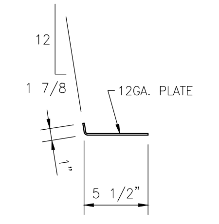
DETAIL OF 'tp3' SCALE: 1 1/2"=1'-0"
